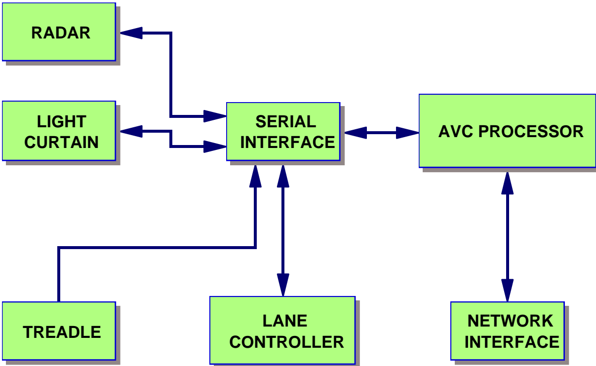
Figure 3.0-1; AVC Block Diagram
