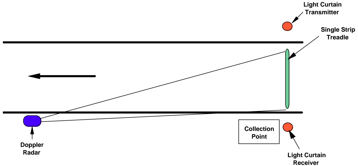
Figure 3.0-2; AVC Lane Sensor Layout
